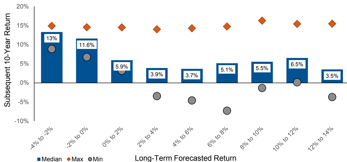
Figure 2. Actual 10-Year Return of Core Assets versus Forecast Based on Historical Returns, 1971-2005 6
