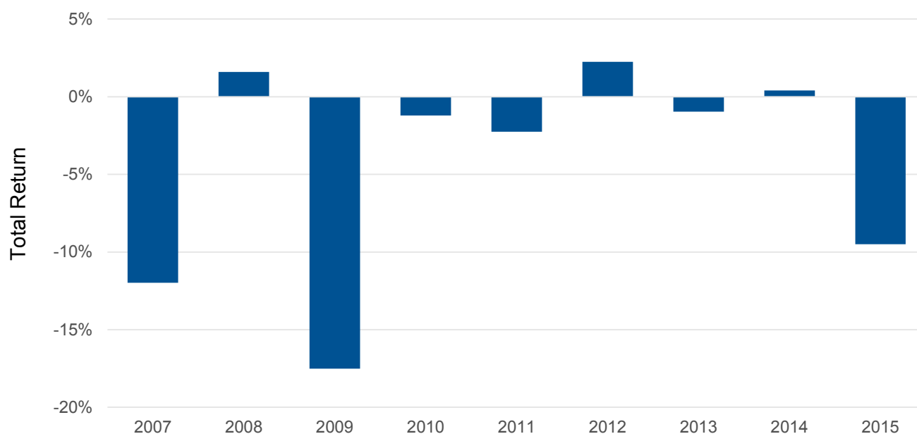
Figure 1. Annual Return of Russell 1000 Value minus Annual Return of Russell 1000 Growth (For the seven years ending December 31, 2009-2015)
