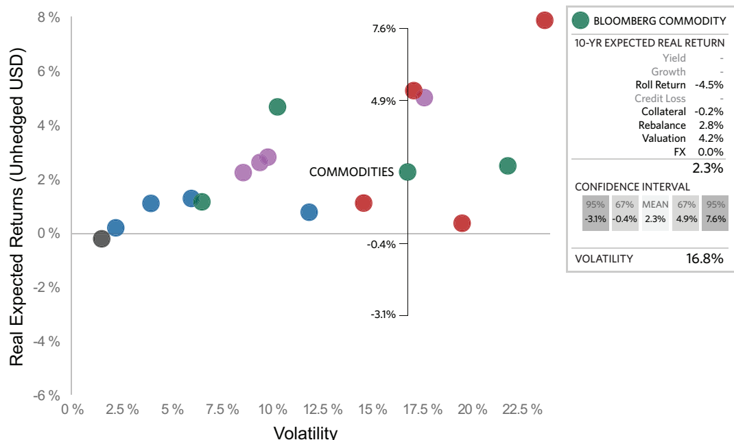
Figure 6. Expected Return and Unexpected Return Variability of Commodities
