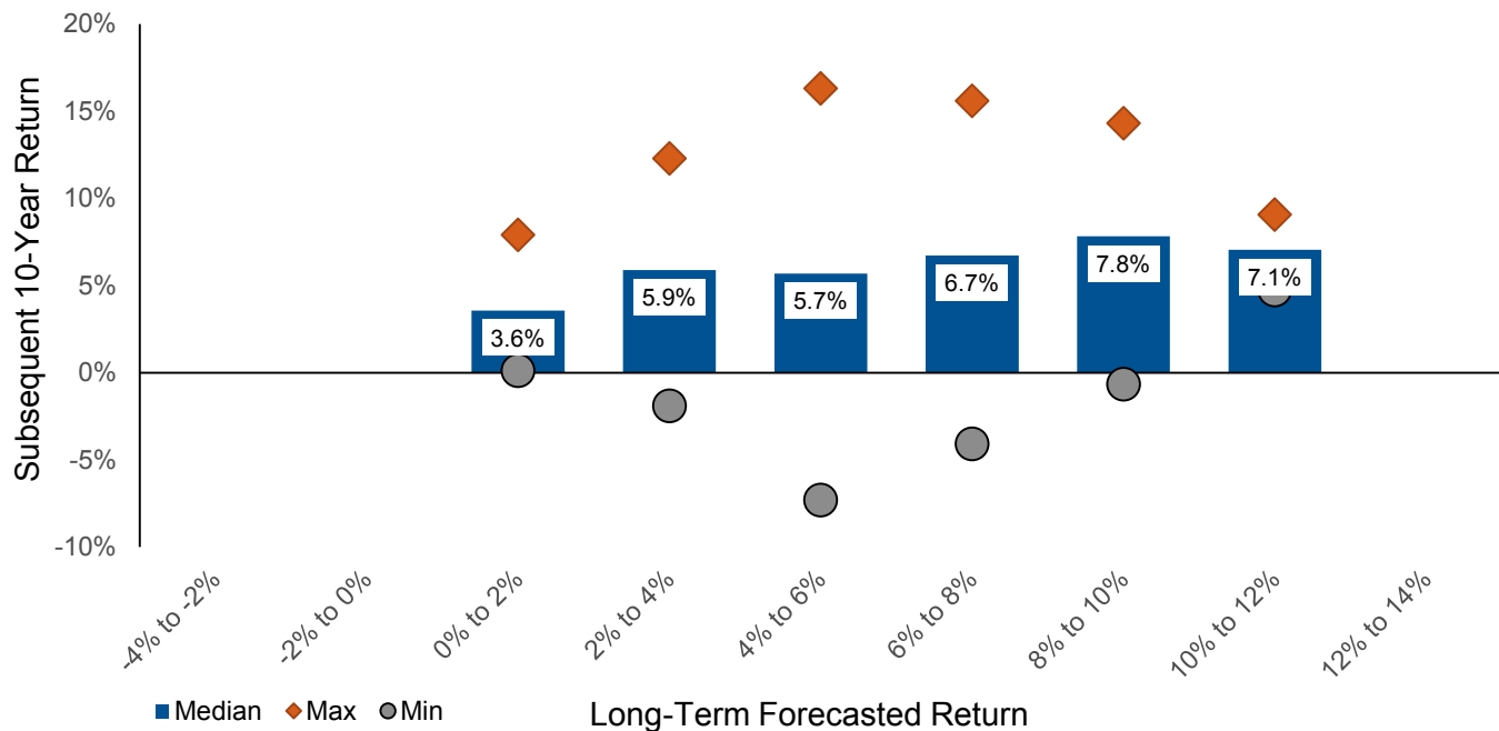
Figure 3. Actual 10-Year Return of Core Assets versus Forecast Based on a Constant Sharpe Ratio, 1971-2005
